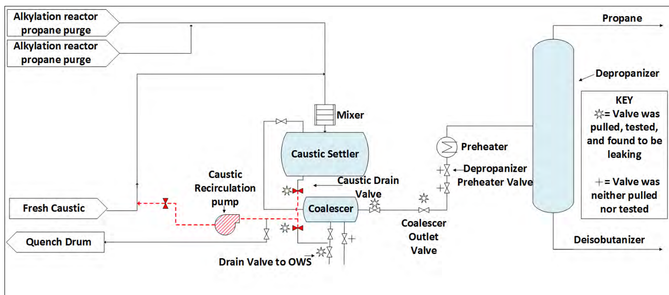
FIGURE 3. Original isolation plan shown in red (Source: CSB).
