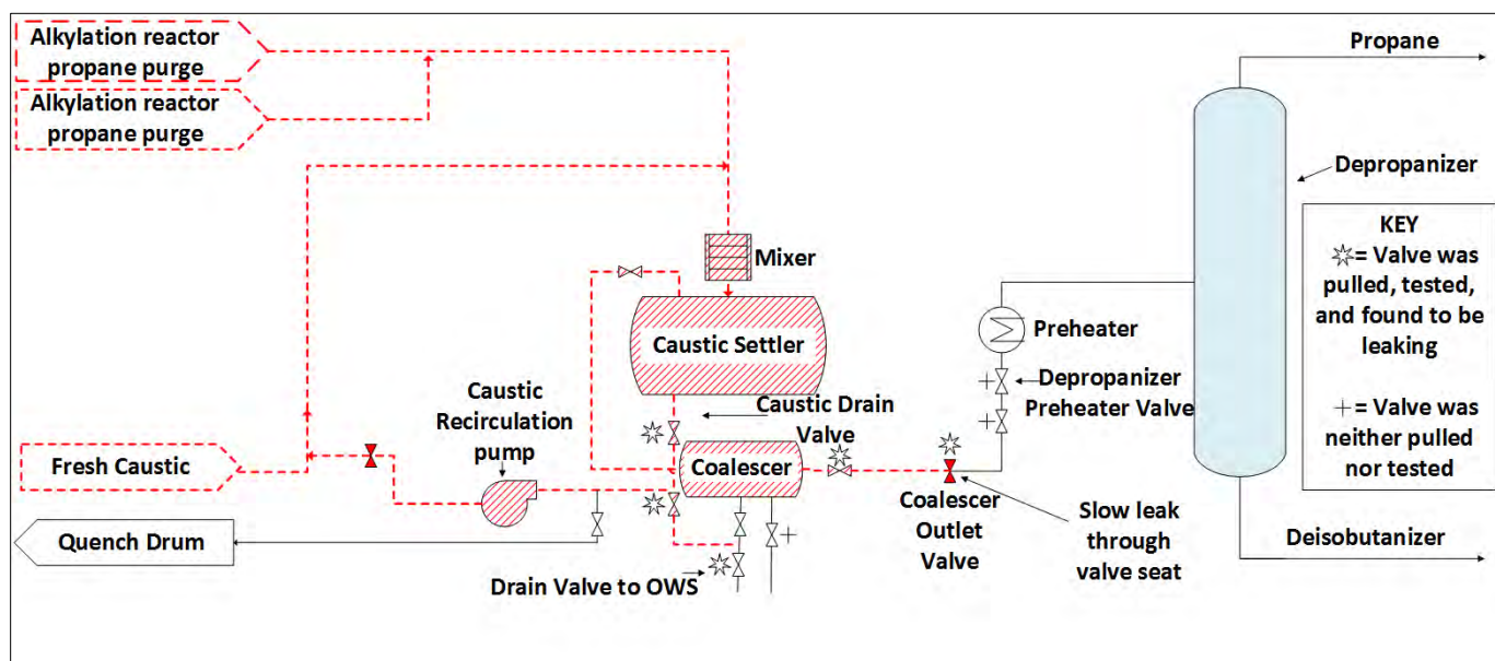
FIGURE 4. Expanded isolation plan shown in red (Source: CSB).
